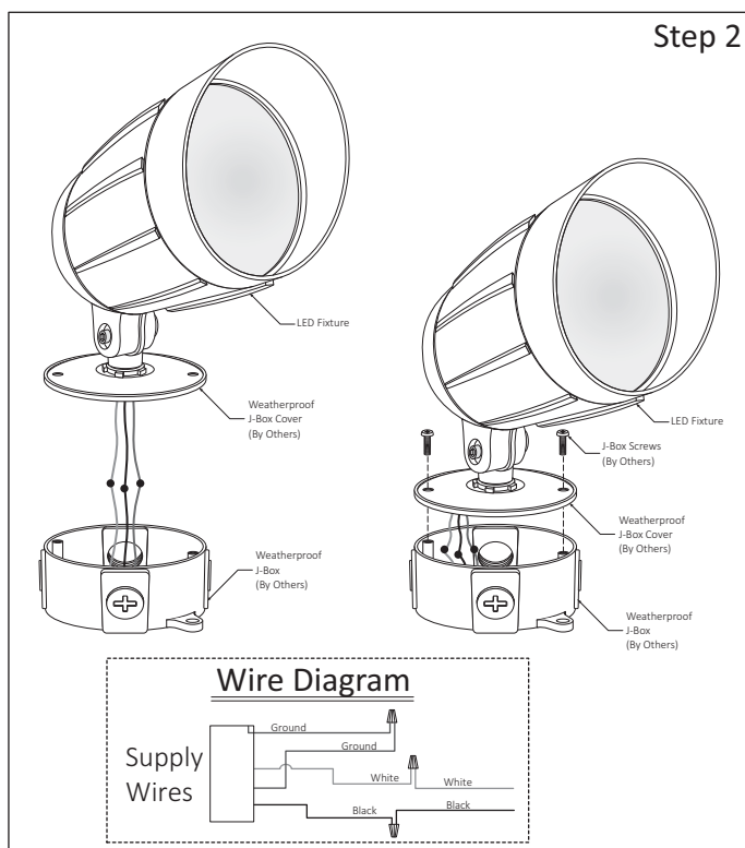
Step 2 - Install Fixture NPT to J-Box Cover: a.- Insert Fixture Input Wires to the threaded hole of J-Box Cover. b.- Screw in the NPT to fasten the Fixture. c.- Make wiring connections, see Wire Diagram. d.- Place J-Box cover and fasten to Weatherproof J-Box (by others).
