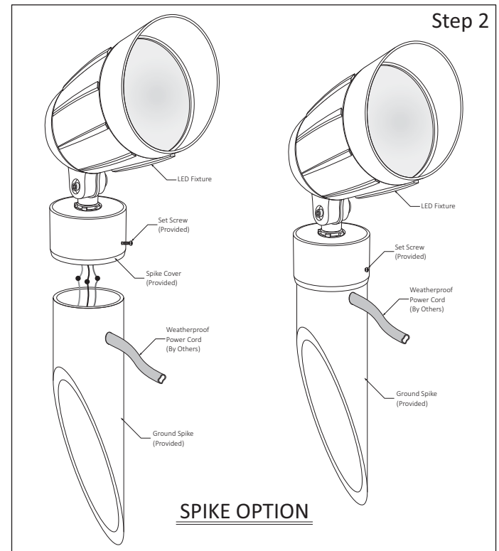
Step 2 - Install Fixture NPT to Spike Cover: a.- Insert Fixture Input Wires to the threaded hole of Spike Cover. b.- Screw in the NPT to fasten the Fixture. c.- Insert Power Cord (by others) and make wiring connections, see Wire Diagram. Use Electrical Tape to protect the connections. d.- Place Spike Cover and fasten by Set Screw (Provided). e.- Run Power cord to connect into a Weatherproof J-Box (by others).
